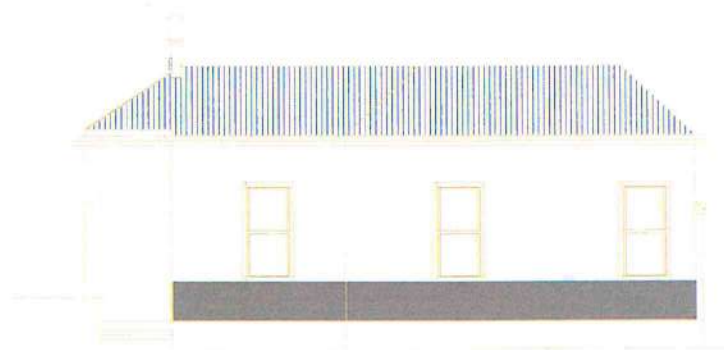
RIGHT ELEVATION SCALE 1:100
