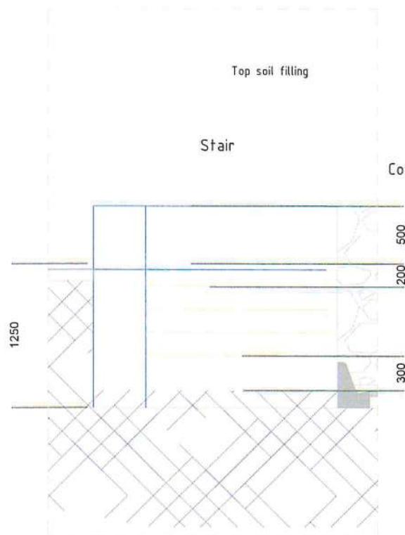
A Detail Stair 01 SCALE 1:50
