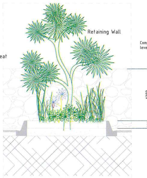
B Detail Garden and Grass Block 01 SCALE 1:20
